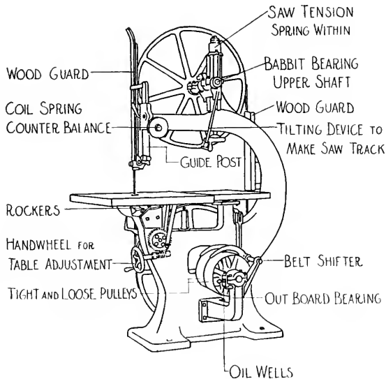
FIG. 181. BAND SAW.
